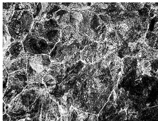
Fig. 5 – Morphology of the carbide phase in high-carbon steel: a – tempered martensite with globular carbides, b – carbide network; a – \times 500 , b – \times 200
