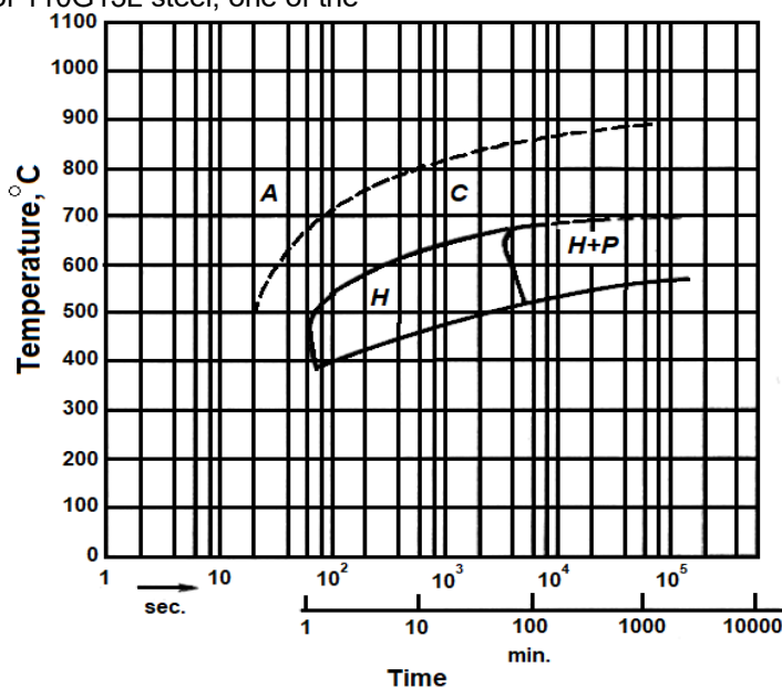
Fig. 1. Thermokinetic diagram of austenitic manganese steel (C – 1.29%, Mn – 13.3%). Austenitization at 1050°C for 15 minutes [9]
