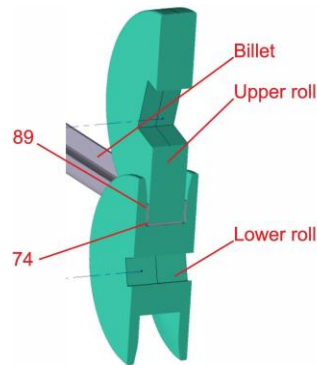
Figure 2 – Cross-section of the final roll stand and characteristic points used for stress–strain state analysis.
