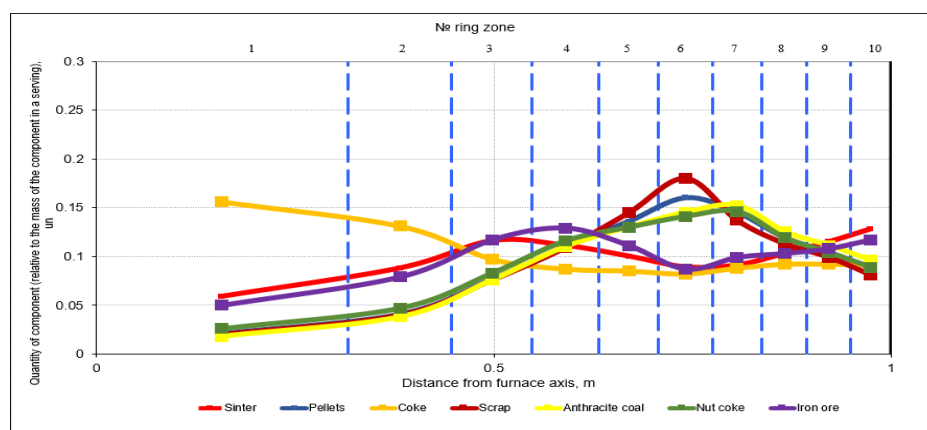
Figure 6 – Mass distribution of charge components along the radius of the to
