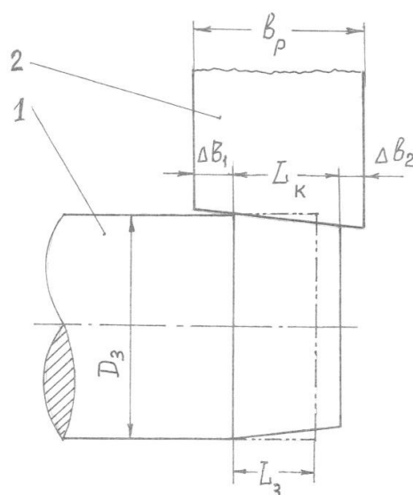
Figure 9 – Diagram of roller contact with the billet at the moment of indentation completion: 1 – billet; 2 – roller
