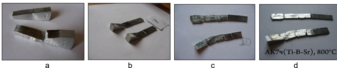
a, b – AK74 alloy of the initial composition; c, d – AK74(Ti-B-Sr) alloy; a, c – casting from 720°C; b, d – thermotemporal treatment ( T=800^\circ\text{C} , t=30 min)
