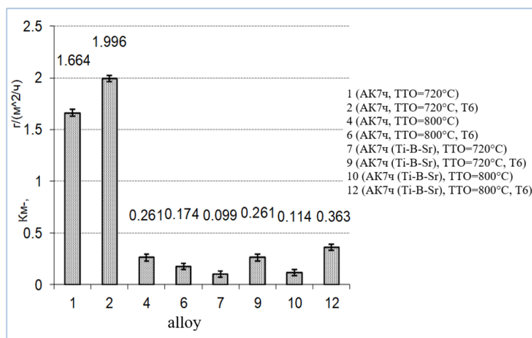
Figure 6 – Corrosion rate of the AK7c alloy of the initial composition and AK7c(Ti-Sr-B) depending on treatment regimes
