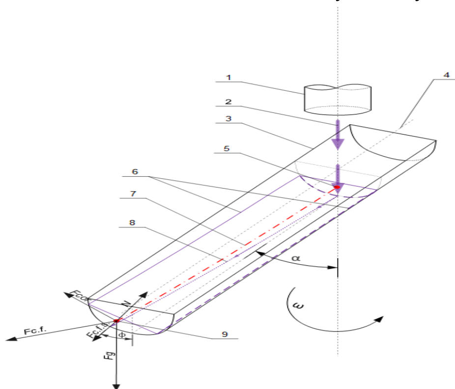
1 - the central pipe of the BLT; 2 - the direction of movement of the charge material; 3 - distribution tray; 4 - longitudinal axis of the tray; 5 - the center of gravity of the flow at the beginning of movement along the tray; 6 - the limits of the flow of charge materials on the tray; 7 - trajectory of the center of gravity of the flow; 8 - the trajectory of the movement of the material point along the tray; 9 - position of the center of gravity of the flow on the unloading end of the tray; \alpha - angle of inclination of the tray to the vertical, degrees; \omega - angular speed of tray rotation, rad/s; \varphi - the angle of lifting (deposition) of materials on the tray, degrees; F_g - gravitational force, N; F_{c.f.} - centrifugal force from tray rotation, N; F_{cor} - Coriolis force, N; F_{c.f.s.} - centrifugal force from lifting (carrying) materials onto the side of the tray, N; N is the normal component of the reaction force, N.
