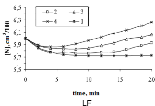
Figure 2. Change in nitrogen concentration in metal at different ratios of argon and nitrogen in the blowing mixture: 1 - argon 0, nitrogen 0.2; 2 - argon 0.1, nitrogen 0.1; 3 - argon 0.2, nitrogen 0 m³/min.
