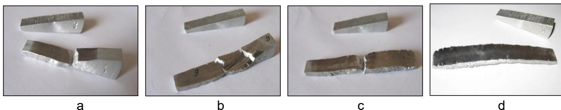
a, b – AK74 of the initial composition; c, d – AK74(Sr-Sc); a, c – cast state; b, d – after hydrogen treatment of the melt for 20 min.
