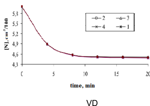
Figure 2. Change in nitrogen concentration in metal at different ratios of argon and nitrogen in the blowing mixture: 1 - argon 0, nitrogen 0.2; 2 - argon 0.1, nitrogen 0.1; 3 - argon 0.2, nitrogen 0 m³/min.
