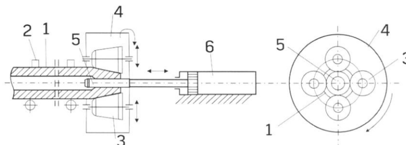
Figure 3 – Preparation of the front end of the shell on a planetary-type rolling machine:
