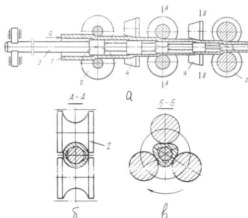
Figure 7 – Scheme of continuous cold pipe rolling [23]:
