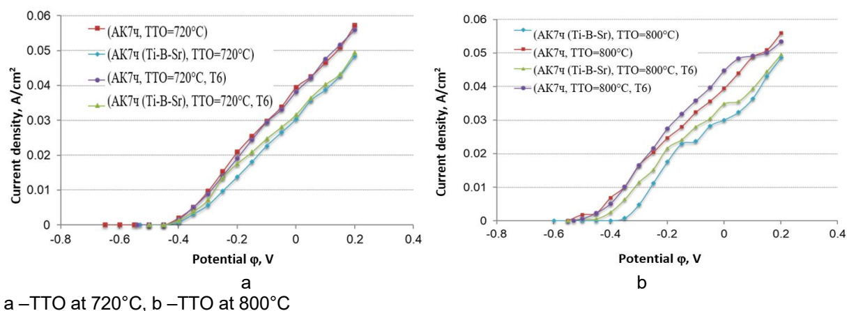
Figure 8 – Polarization curves of AK7c and AK7c(Ti-Sr-B) alloys in the additionally heat-treated state after testing in an aqueous solution of 3% NaCl + 1% HCl
