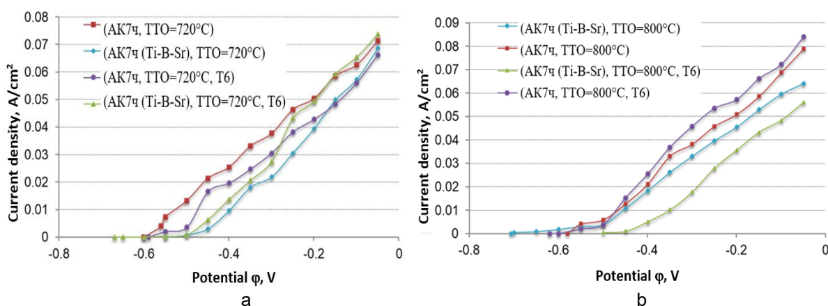
Figure 7 – Polarization curves of AK7c and AK7c(Ti-Sr-B) alloys in the additionally heat-treated state after testing in 0.1 M NaCl solution
