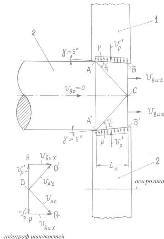
Figure 11 – Slip-line field at maximum indentation of two diametrically opposed rollers and velocity hodograph: 1 – roller; 2 – billet
